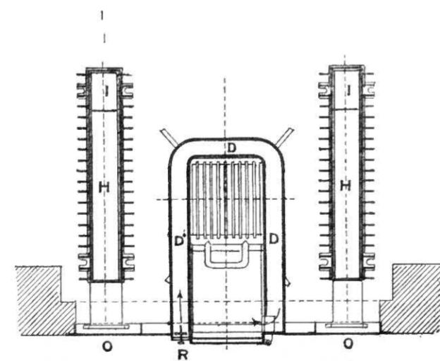
Fig. 497.—Plan of Calorifer.
