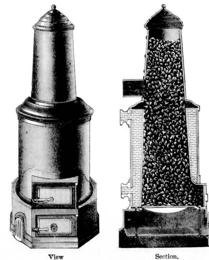
Fig. 503.—View and Section of Independent Conical Boiler.
