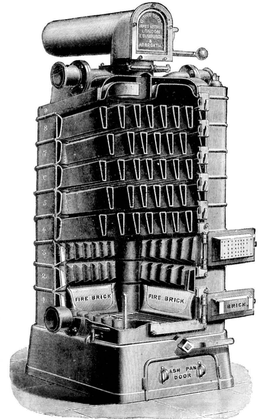
Fig. 515.—Sectional View of the "Challenge" Cast-iron Boiler.
