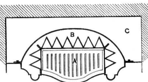
Fig. 467.—Plan and Front View of Boyd's Warm-air Grate.
