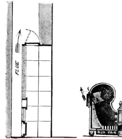
Fig. 452.—Section of Nautilus Grate.
