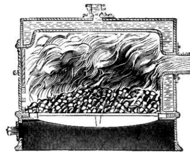
View. Fig. 507.—View and Section of Independent Saddle Boiler.
