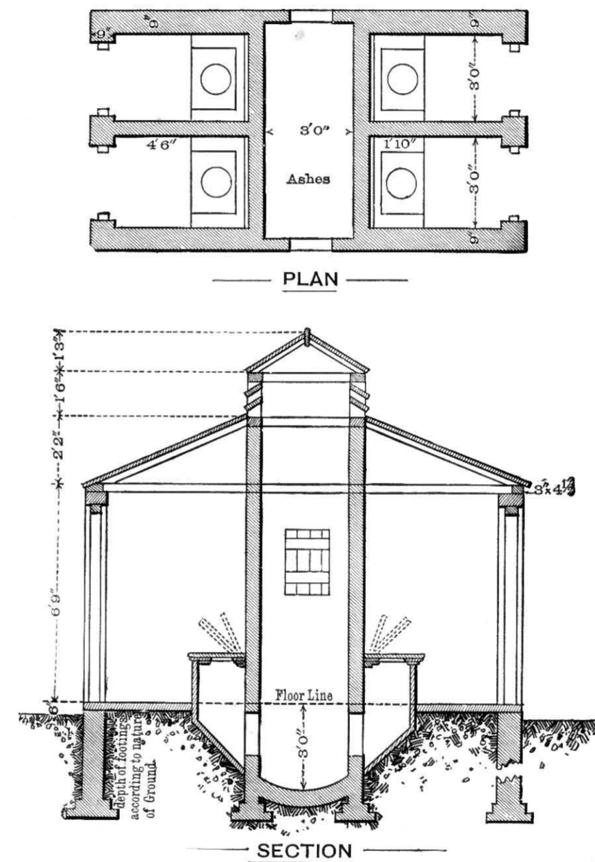
Fig. 434.—Plan and Sections of Midden-closet formerly used in Manchester.
