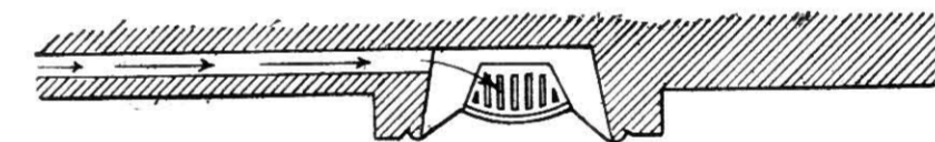
Fig. 450.—Plan of Fire-grate, with Special Air-duct.
