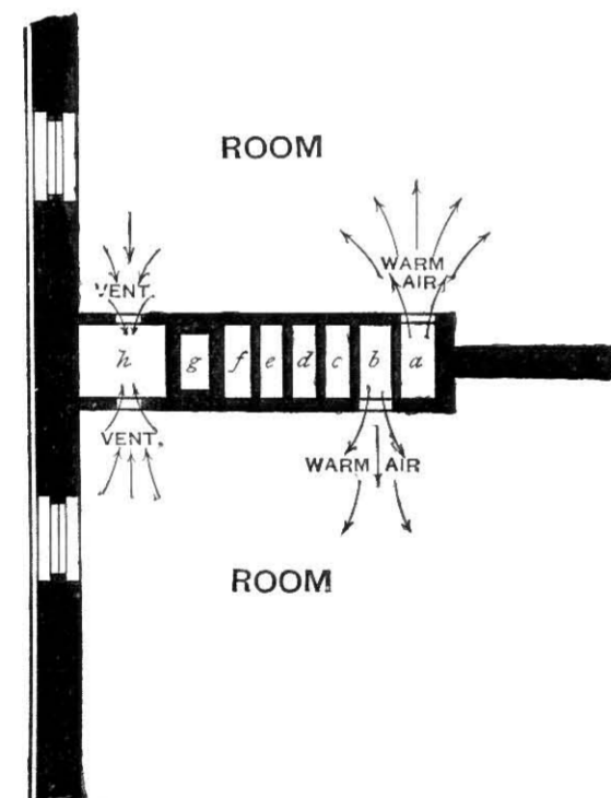
Fig. 492.—Plan showing Stack of Inlets and Outlets, "Smead" System.
