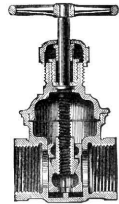
Fig. 532.—Section of Full-way "Peet" Valve.
