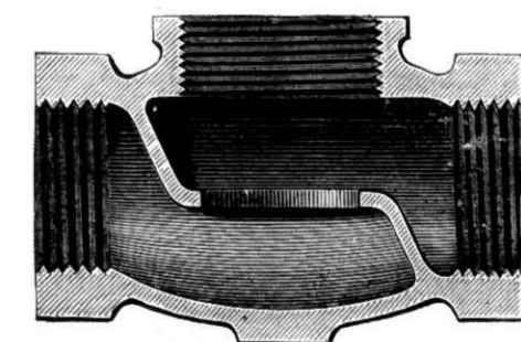
Fig. 554.—Dewrance's Renewable Valve.
