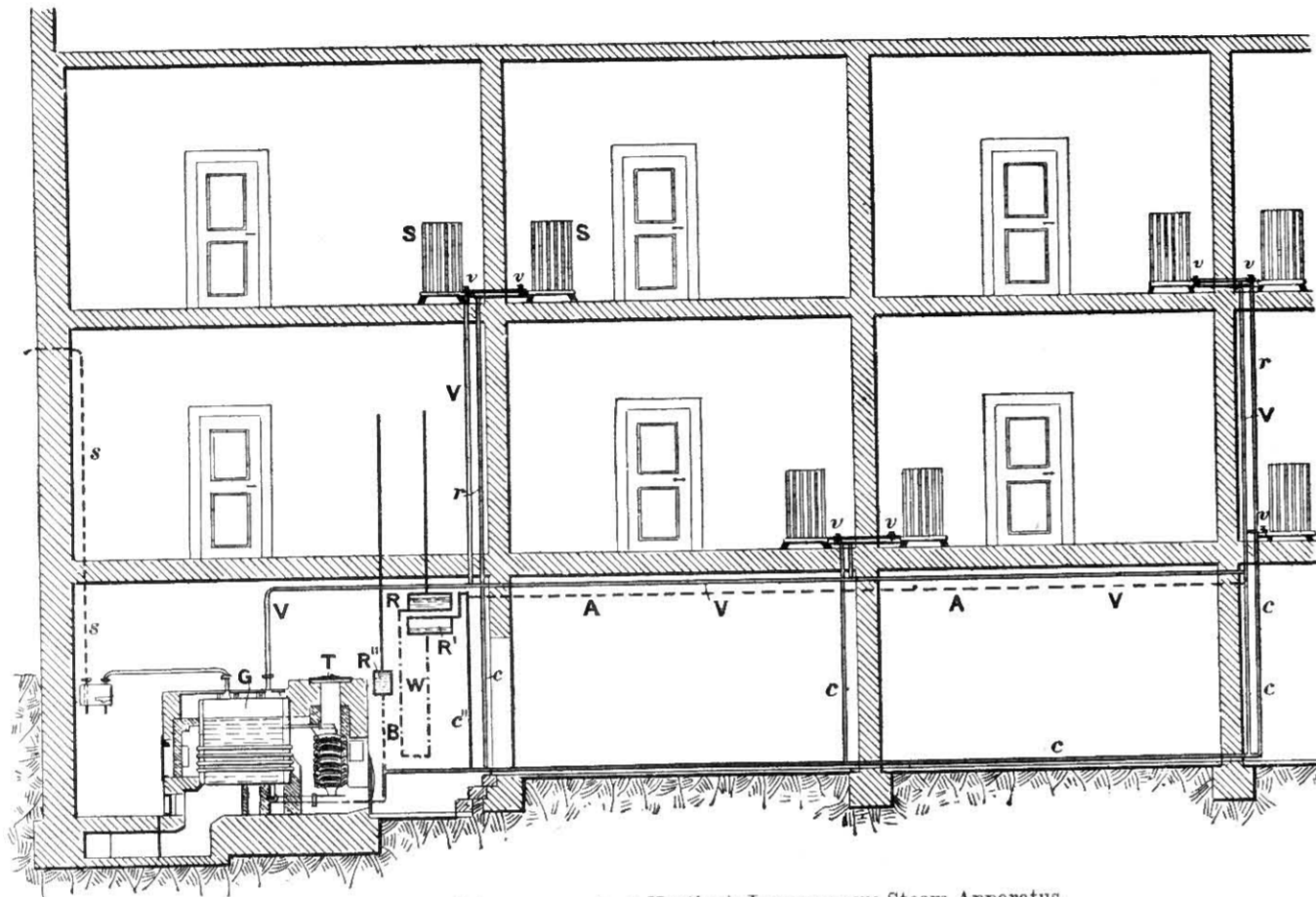
Fig. 551.—General Arrangements of Körting's Low-pressure Steam Apparatus.
