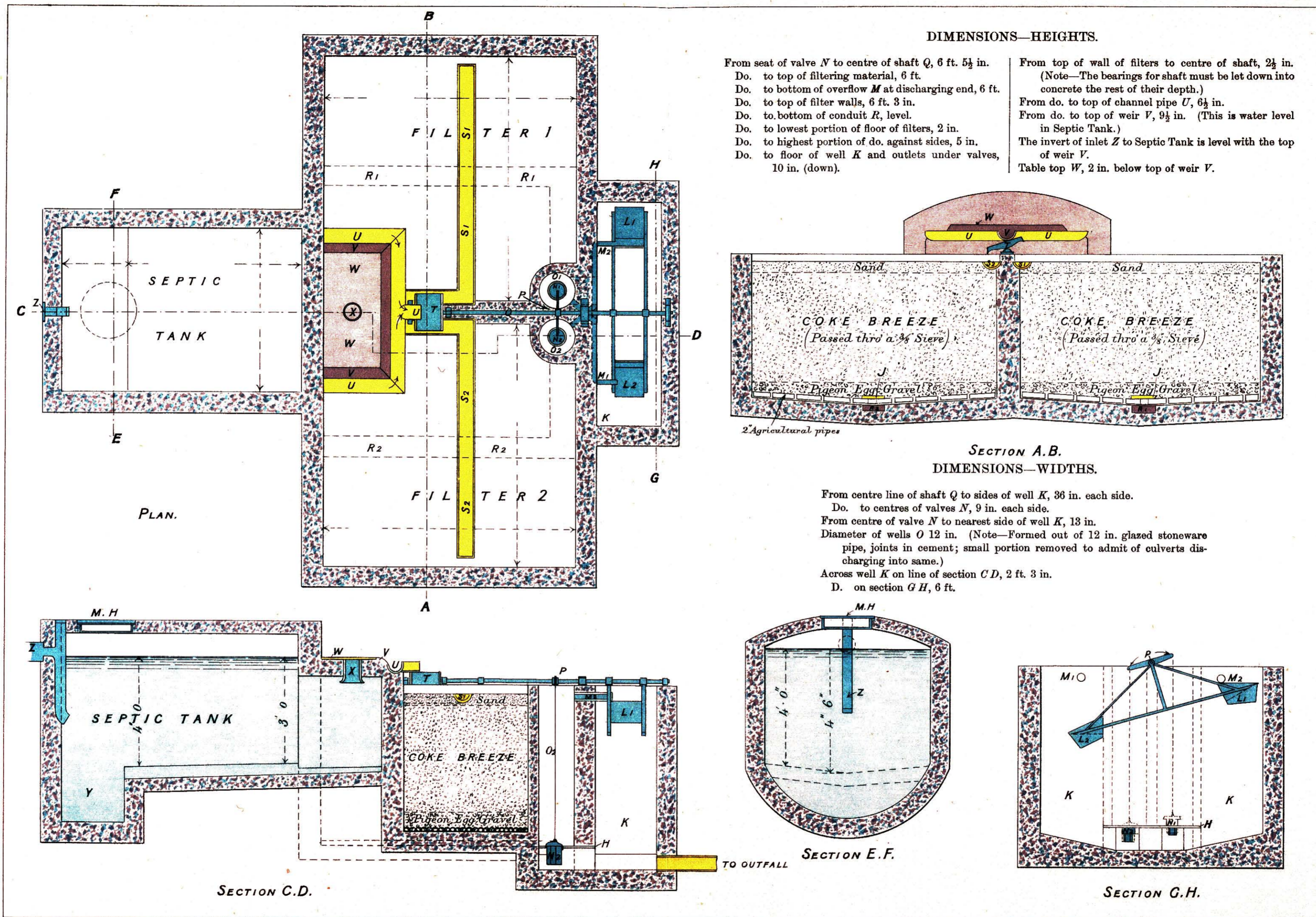
THE SEPTIC TANK SYSTEM OF SEWAGE TREATMENT, SHOWING FILTERS AND ALTERNATING GEAR.
