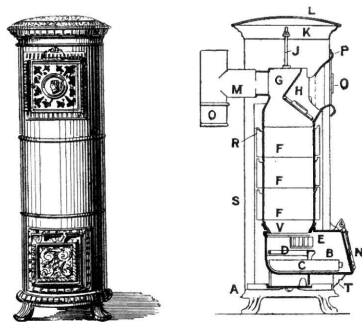
Fig. 470.—View and Section of the "Hestia" Stove.
