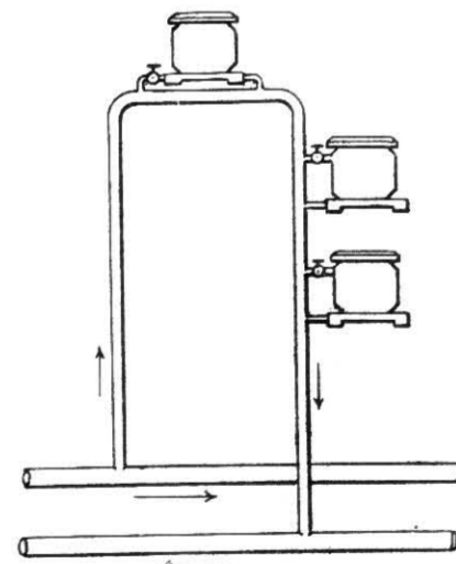
Fig. 539.—Radiators on Branch Circulation-pipe.
