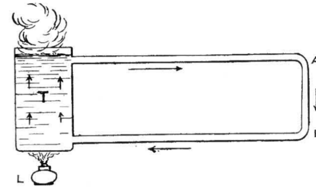
Fig. 534.—Simplest System of Low-pressure Heating.
