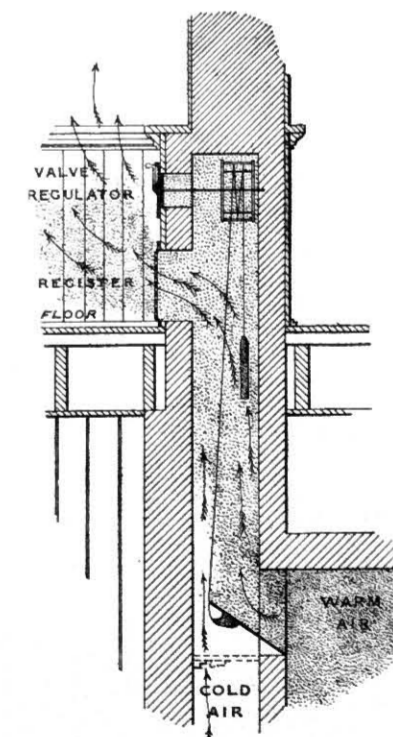
Fig. 494.—Section of Duct showing Valve for Incoming Air.
