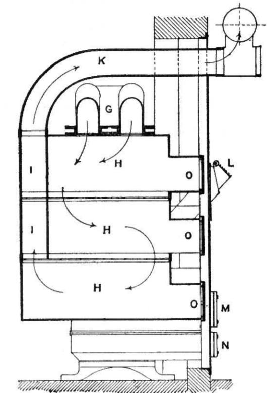
Fig. 498.—Vertical Section through Radiator of Calorifer.
