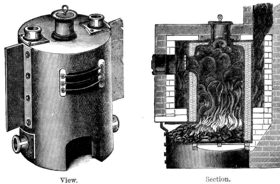
Fig. 505.—View and Section of the "Excelsior" Boiler.
