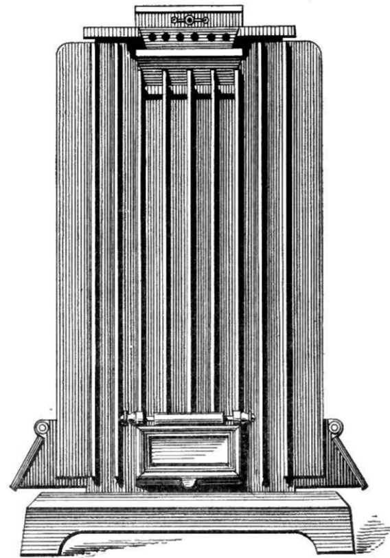
Fig. 473.—Front Elevation of One-chambered Controlled-combustion Heating Apparatus.
