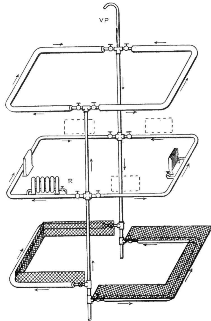
Fig. 526.—Diagrammatic View of Low-pressure Hot-water Pipes R, radiator; VP, vent-pipe.
