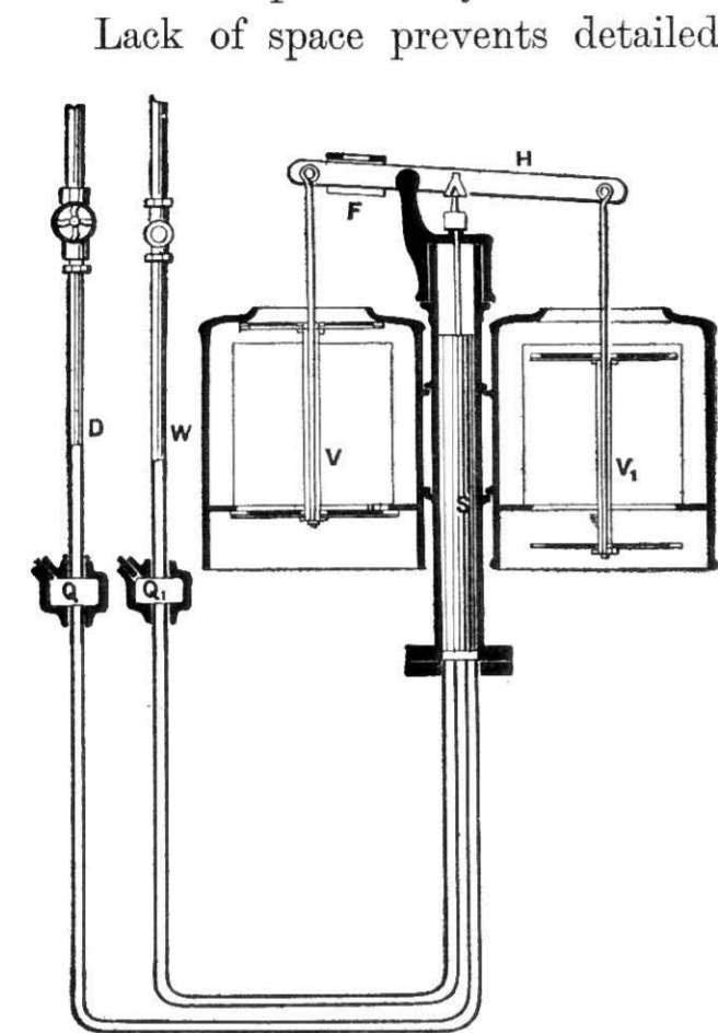
Fig. 519.—Section of Körting's Automatic Draught-regulator.
