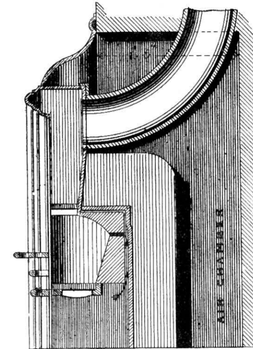
Fig. 456.—Section of Galton Grate.
