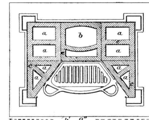
Fig. 457.—Plan of the Galton Independent Stove.
