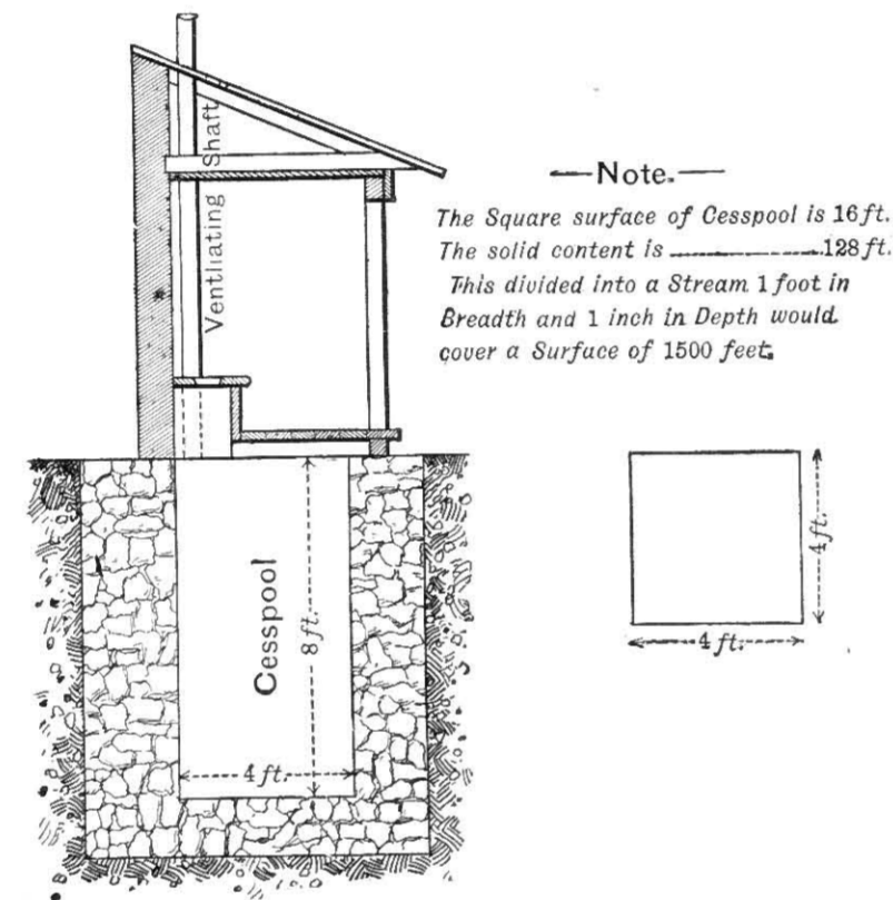
Fig. 430.—Section of insanitary Privy and Cesspool.
