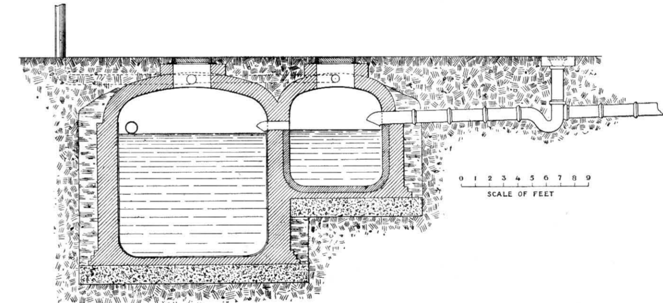
Fig. 442.—Section of Double Cesspool.
