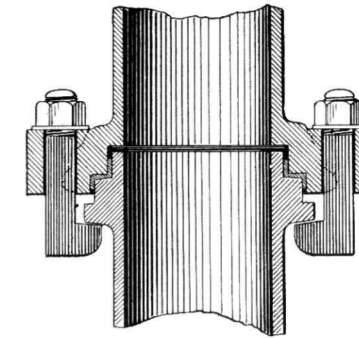
Fig. 521.—Section of Richardson's India-rubber Expansion-joint.
