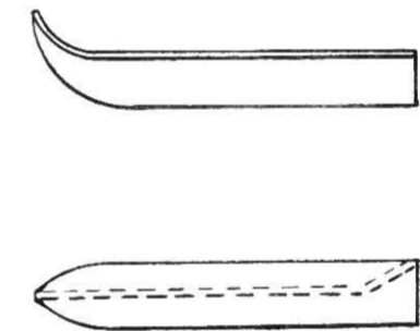
Fig. 525.—Elevation and Plan of T-iron Bracket for Pipes.
