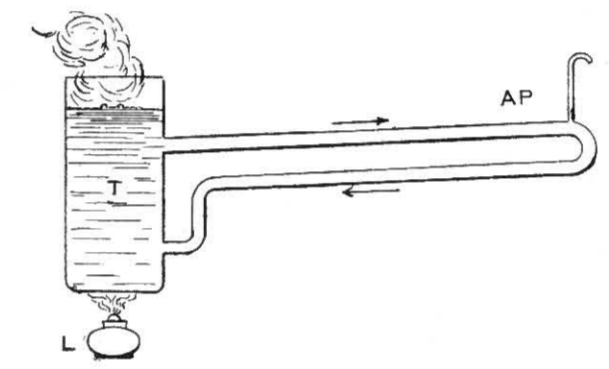
Fig. 535.—Simple Low-pressure Hot-water Apparatus with Air-pipe.
