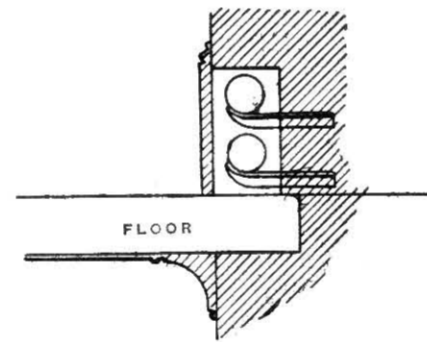
Fig. 527.—Pipes in Channel formed in Wall.
