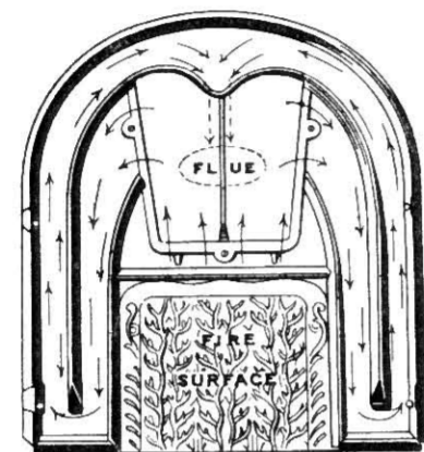
Fig. 479.—Section of Gas-stove with Flues for Utilizing the Waste Heat.
