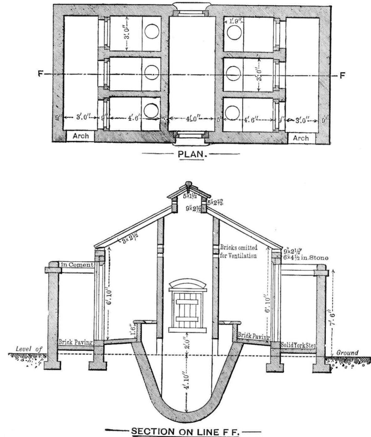
Fig. 431.—Plan and Section of Midden-closet in use at Nottingham.
