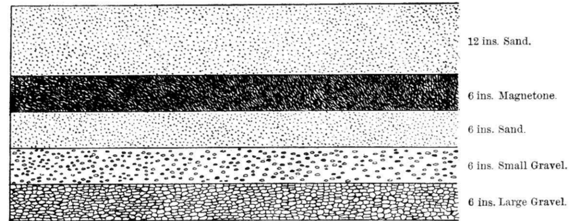
Fig. 426.—Section of Sewage-filter composed of Sand, Gravel, and Magnetone.
