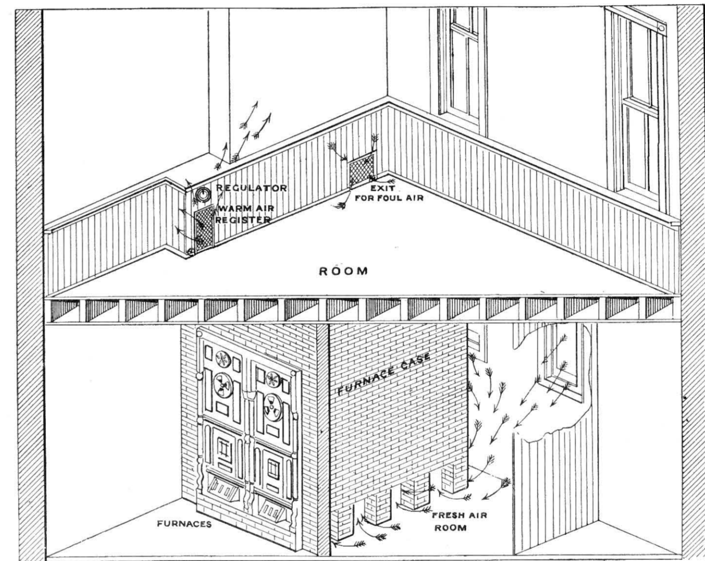
Fig. 490.—View of "Smead" Furnace set in Brickwork.
