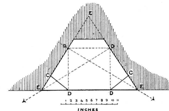
Fig. 461.—Plan of Teale Fire-grate.
