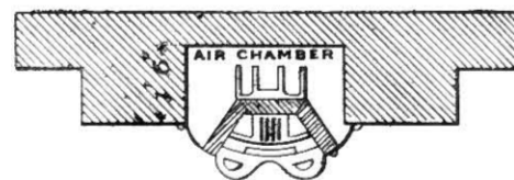
Fig. 453.—Plan of the Galton Grate.
