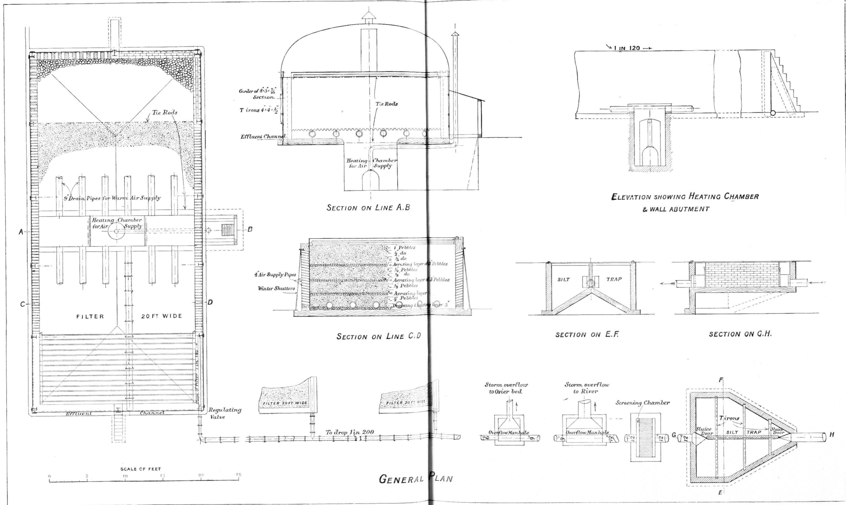
COL. DUCAT'S AËRATED BACTERIAL SEWAGE-FILTER.
