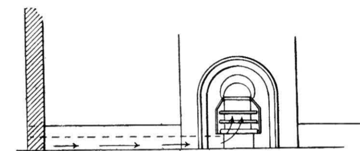
Fig. 449.—Elevation of Fire-grate, with Special Air-duct.
