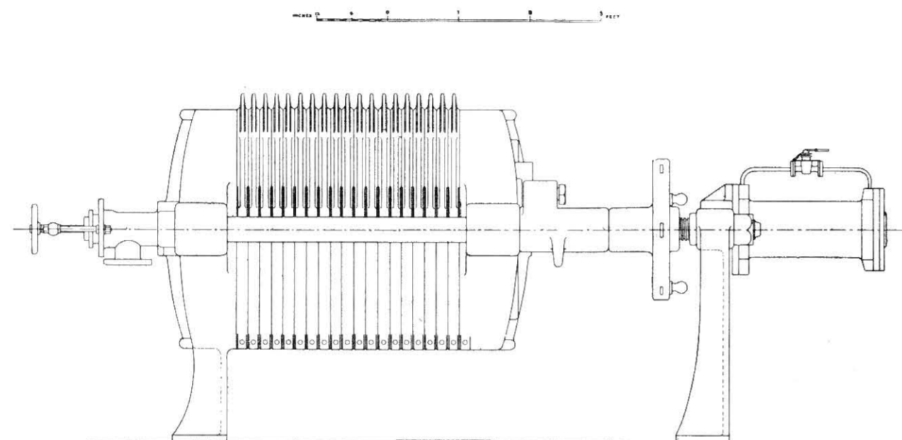
Fig. 425.—Elevation of Manlove and Alliott's Filter-press for Sewage Sludge.
