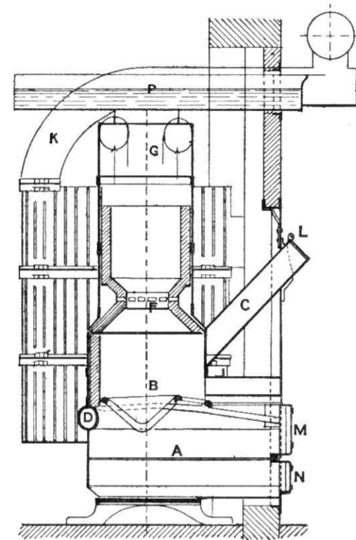
Fig. 495.—Vertical Section of Calorifer from Back to Front.
