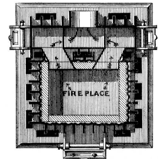
Fig. 471.—Plan of One-chambered Controlled-combustion Heating Apparatus.
