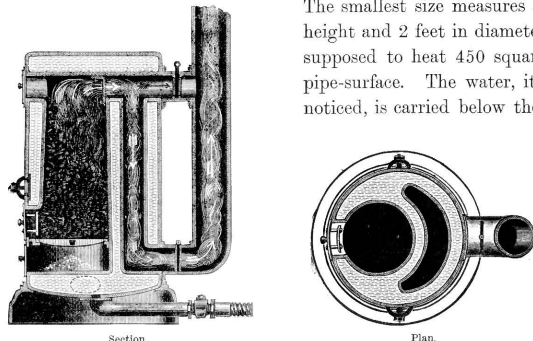
Fig. 504.—Plan and Section of the "Marlor" Boiler.
