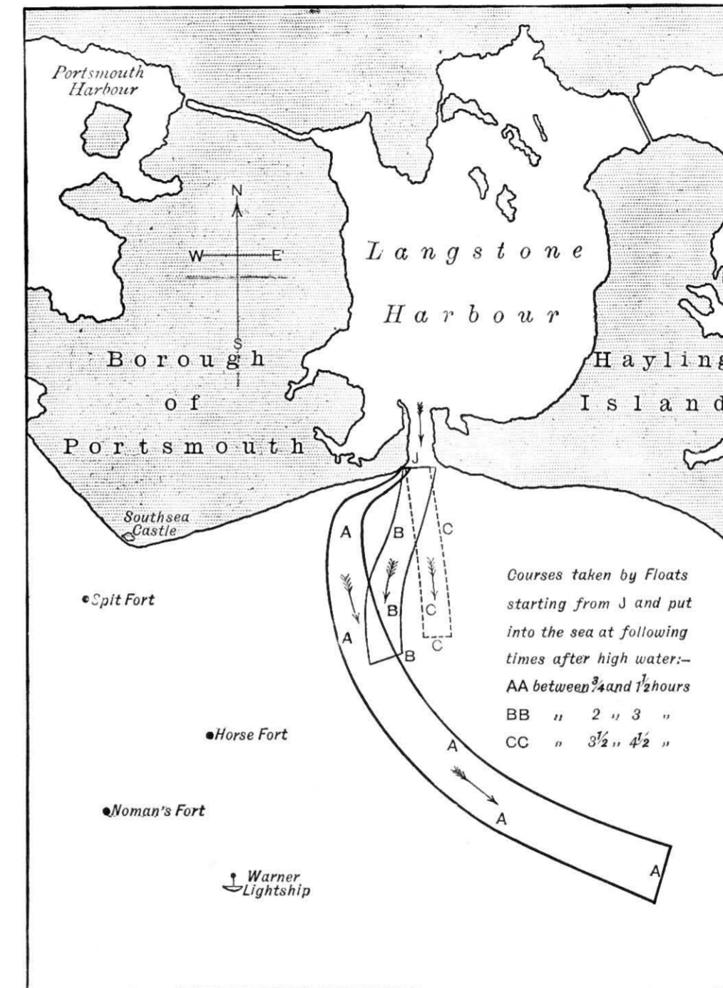
Fig. 424.—Borough of Portsmouth: Sewage-outfall Works. Plan showing float-observations taken from the outfall.
