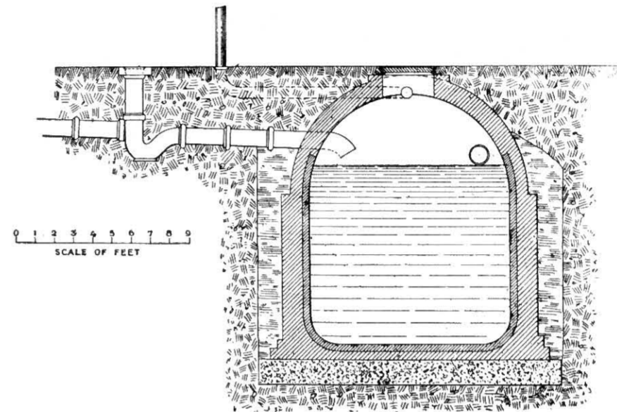
Fig. 441.—Section of Circular Cesspool.
