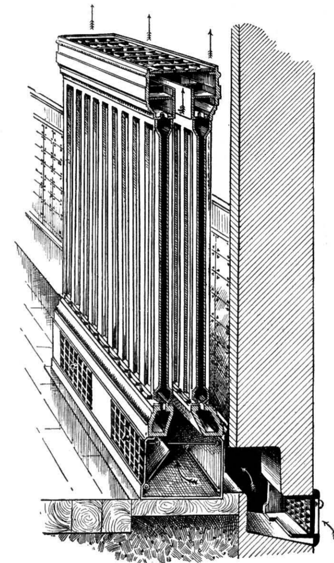
Fig. 531.—Sectional View of Rosser & Russell's Ventilating Radiator.
