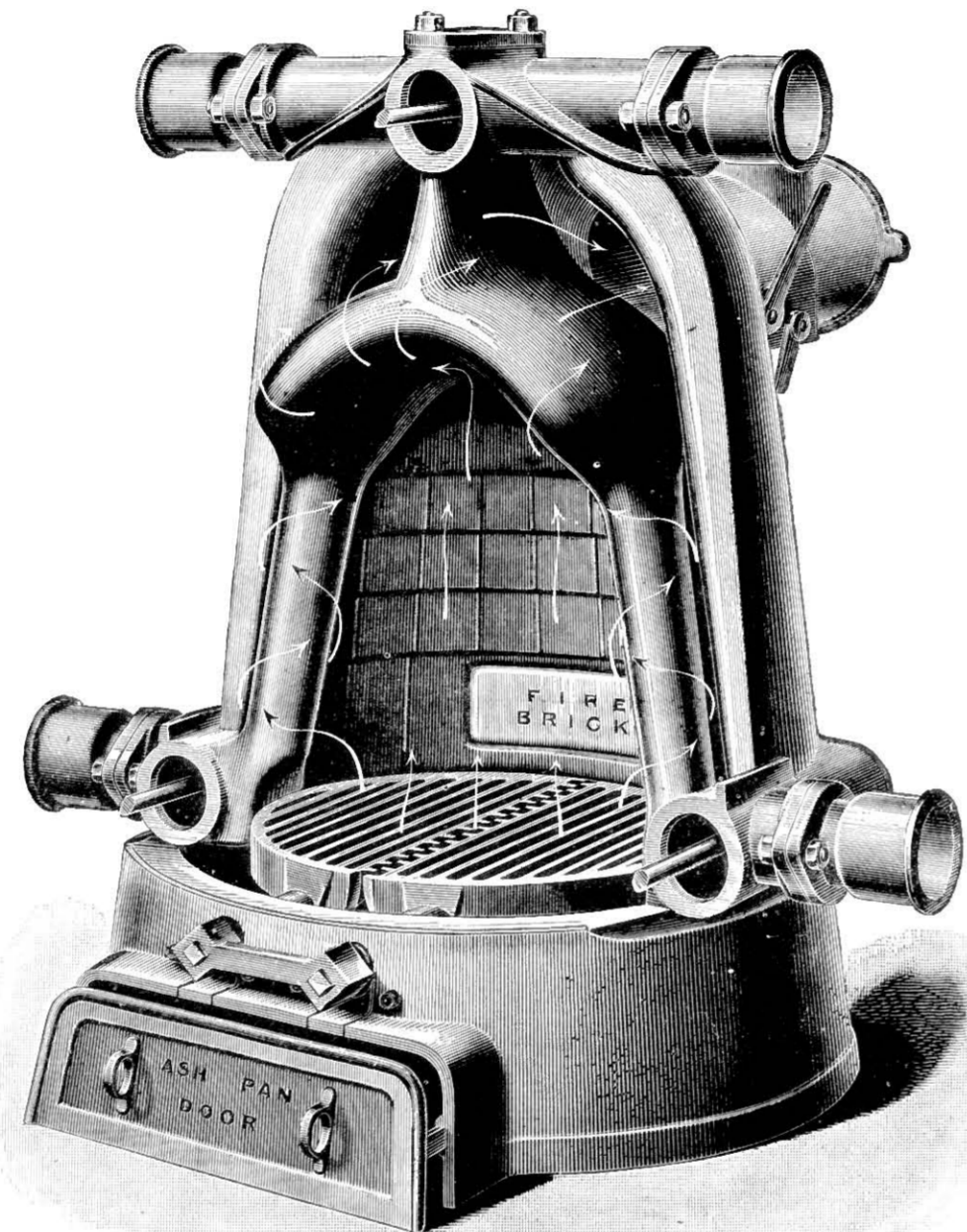
Fig. 514.—View of "Viaduct" Cast-iron Boiler, with the Front Half of the Outer Case Removed.
