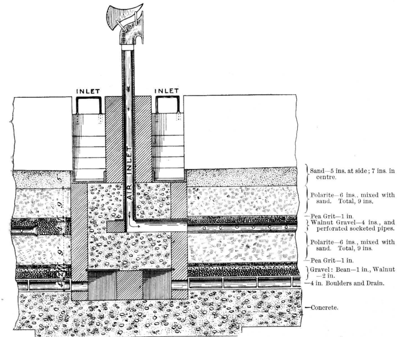
Fig. 427.—Section of Part of a Polarite Sewage-filter.
