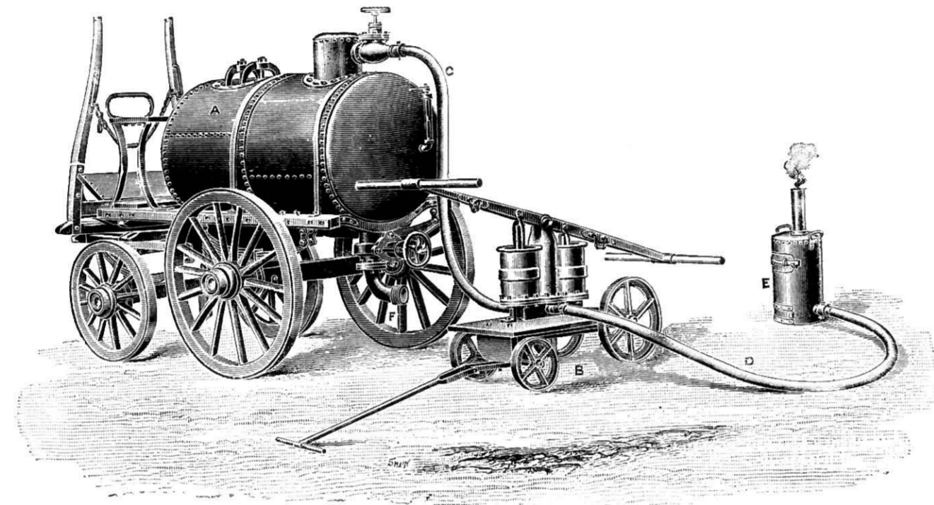
Fig. 443.—Merryweather's Pneumatic Cesspool-emptier.
