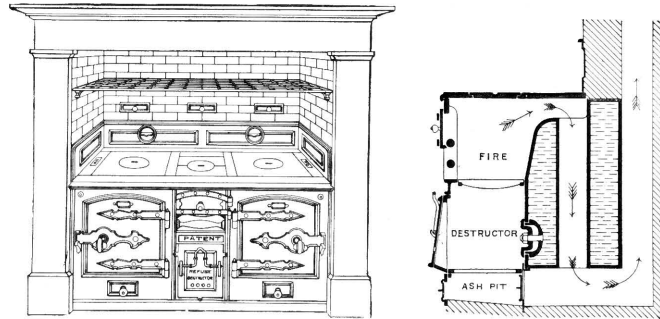
Fig. 476A. — View of Petter's Patent Refuse-destroyer, with enlarged Section through Destructor and Fire-grate.
