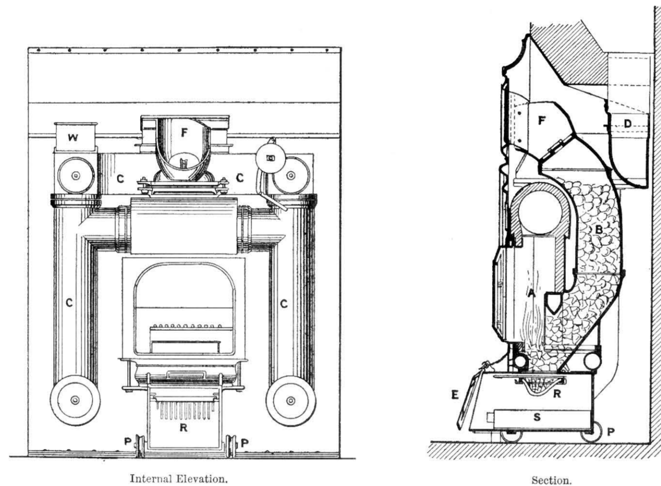
Fig. 468.—The "Helios" Smoke-consuming Stove.
