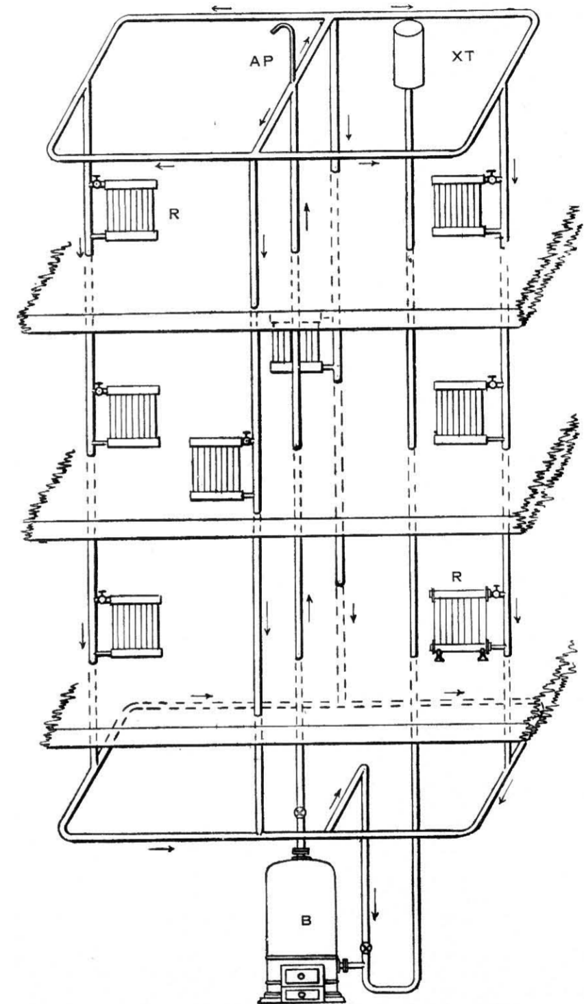
Fig. 543.—Diagrammatic View of the "Mills" System of Piping for Low-pressure Hot-water Apparatus. B, boiler; R R, radiators; AP, air-pipe; XT, expansion-tank.
