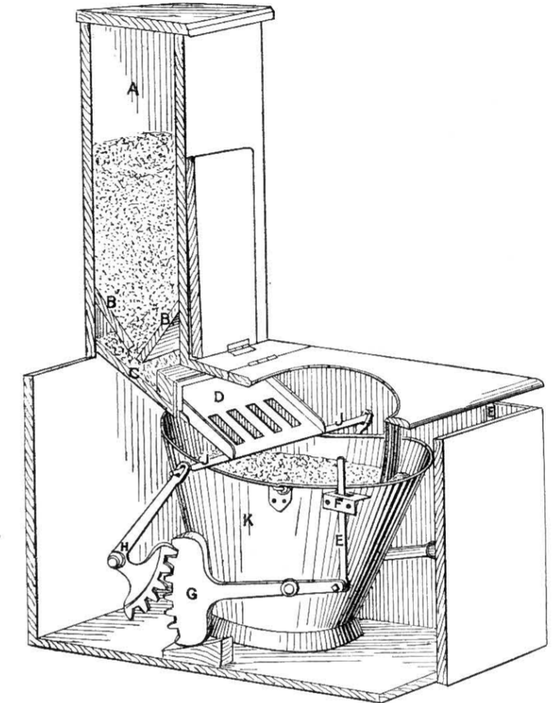
Fig. 446.—Sectional View of the British Sanitary Company's Self-acting Earth-closet.
