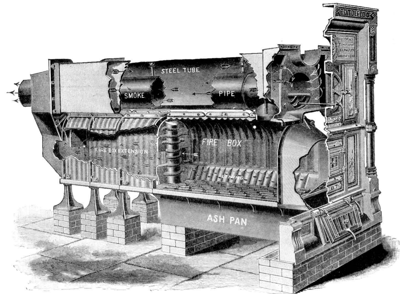
Fig. 489.—The "Smead" Furnace.
