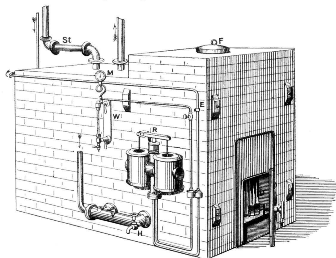
Fig. 517.—View of Exterior of Körting's Boiler.
