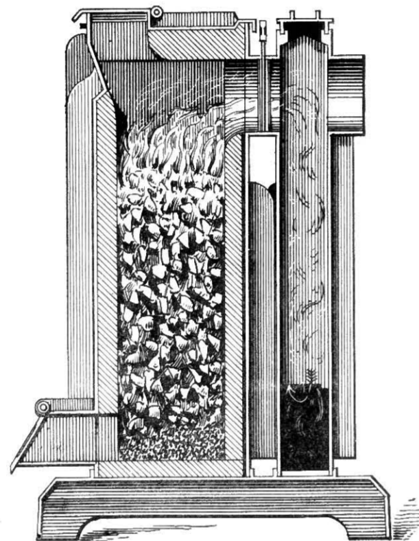
Fig. 472.—Vertical Section of One-chambered Controlled-combustion Heating Apparatus.
