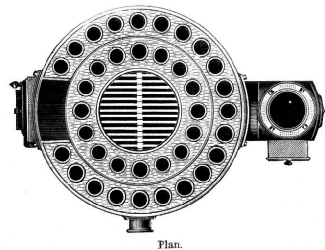
Fig. 547.—Elevation, Section, and Plan of the "Majestic" Independent Boiler for Steam-heating.
