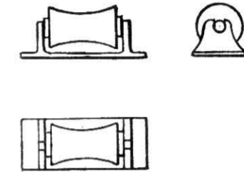
Fig. 522.—Front and End Elevations and Plan of Roller Stool for Pipes.
