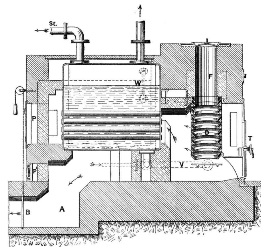
Fig. 518.—Section of Körting's Boiler.
