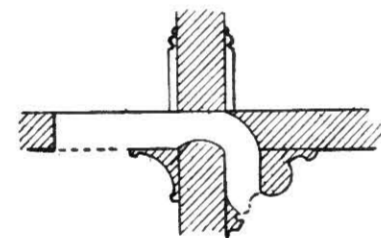
Fig. 500.—Section showing Air-inlet from Corridor to Room.
