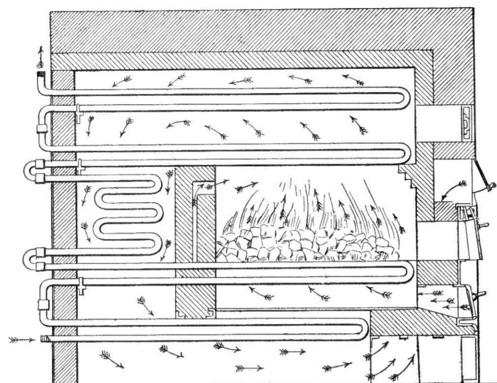
Fig. 516.—Section of the "Renton Gibbs" Tubular Boiler.
