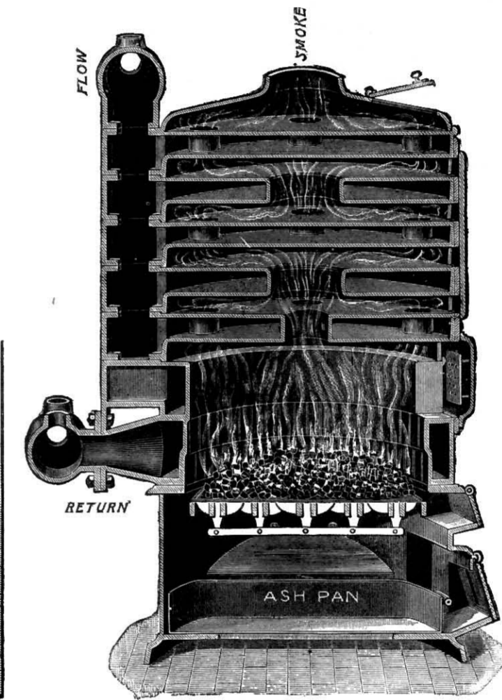
Fig. 510.—View and Vertical Section of the "Oxford" Cast-iron Boiler.
