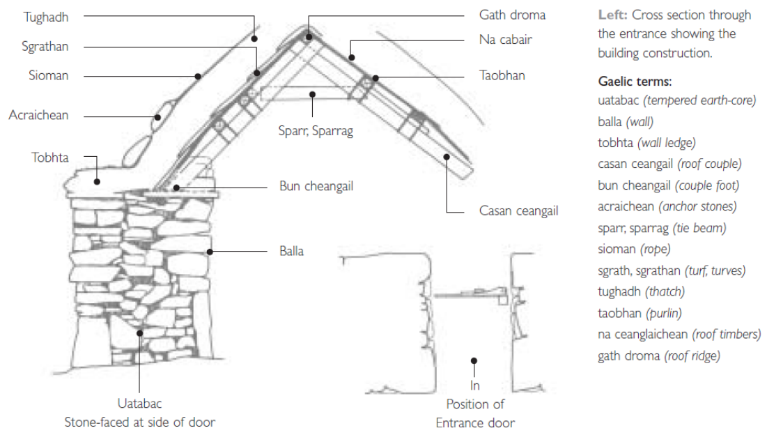
Diagram showing Gaelic terminology of parts of the blackhouse
