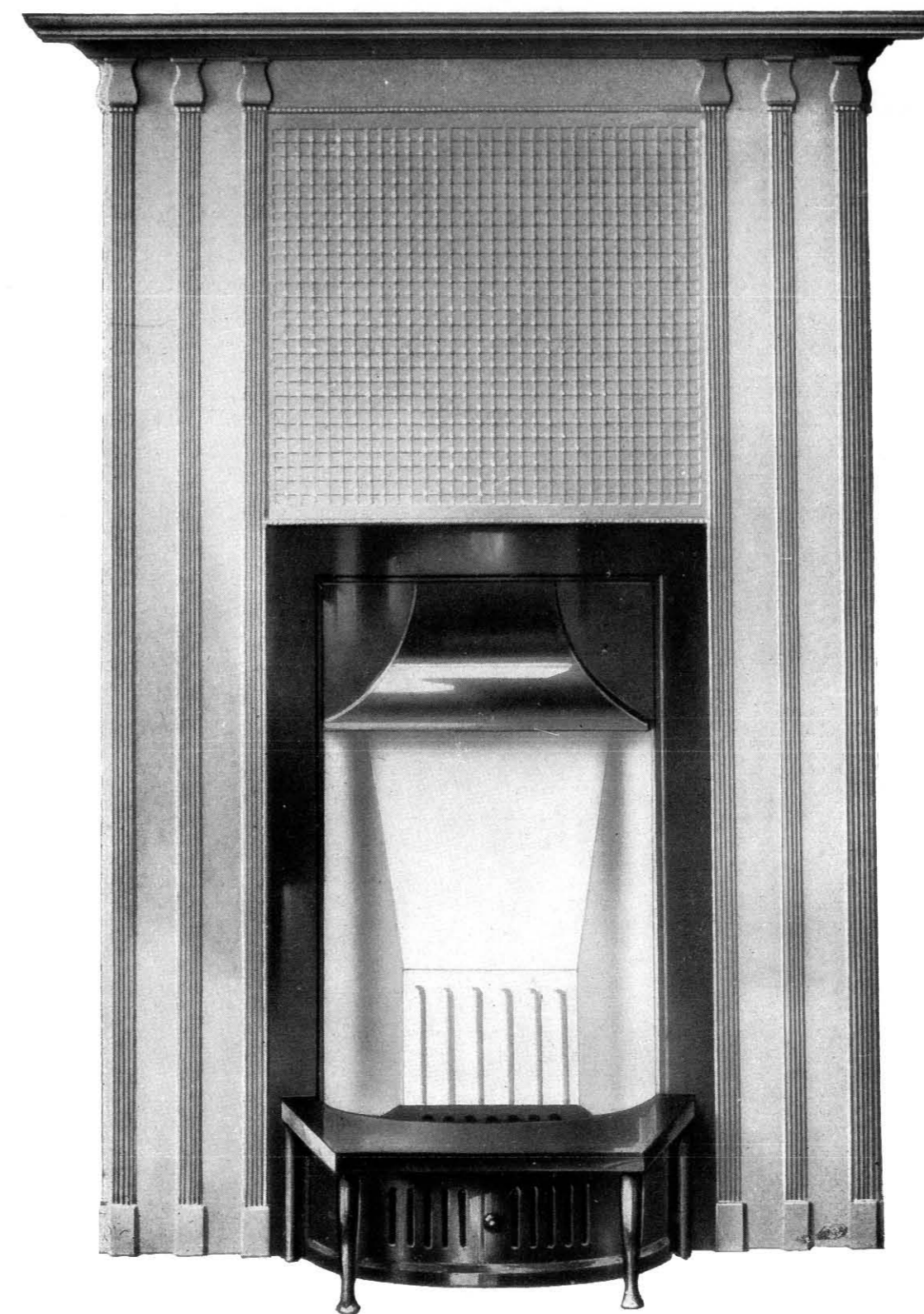
No. 748 MANTEL GRATE, with Double Shelf, Adjustable Cast-iron Canopy, "Alpha" Fire with Sliding Draught Regulator and No. 35 Trivet Hob, Brick Back in four pieces.
