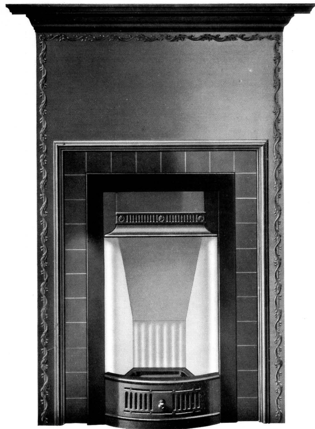
No. 810 TILE MANTEL GRATE, with Single Shelf, Adjustable Cast-iron Canopy, Brick Back in four pieces, "Douglas" Fire, with Sliding Draught Regulator. Prepared for 3 in. Tiles.
