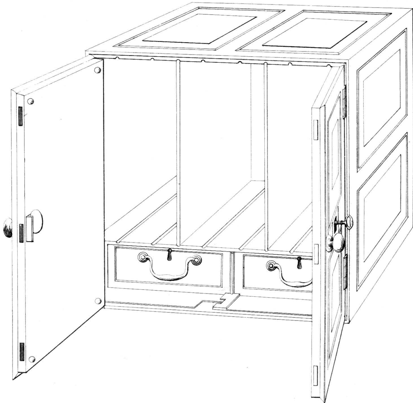
Book Case with double doors, drawers & sliding partitions.
