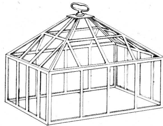
Hand Glass Frame.
