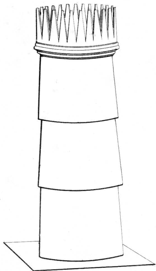
Chimney Cars 1. 33 1/2 ins. high, 10 in diameter at top, 13 1/2 ins. square at bottom. 2. 40 " " " " " " " " " " " "
