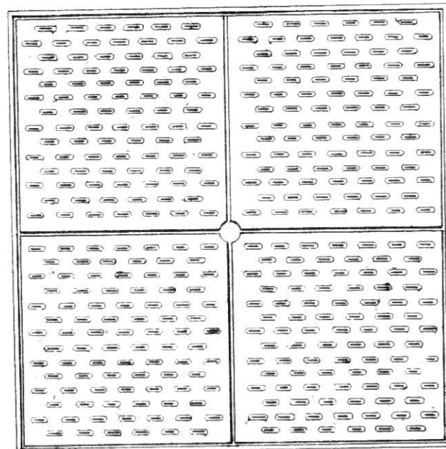
Kiln Plate with long holes. Size 18 Inches square.
