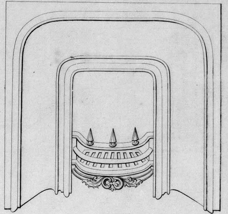
Sham Kinnaird Stove N o 180 with N o 7 bars. Sizes, 30-32-34 x 36-36-38 x 38 & 40 x 40 ins.
