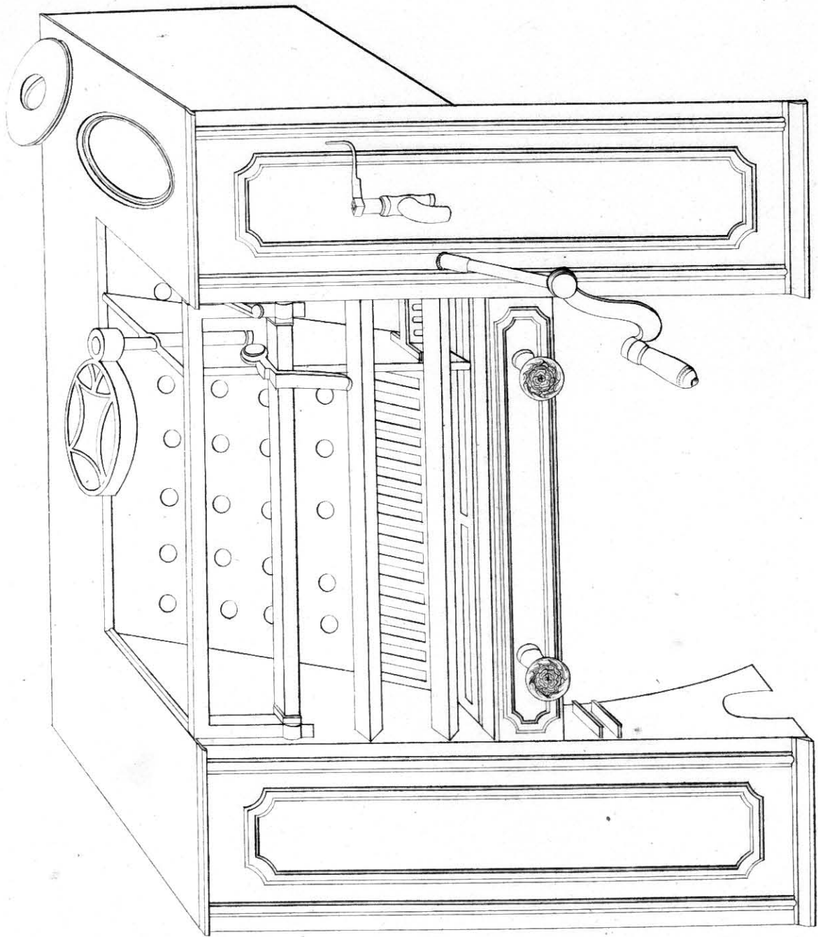
Back Boiler Range with plain Front,
