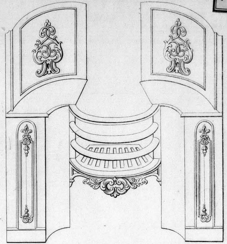
Leith Concave Sham Stove 18 ins. high with Covers Sizes 24 up to 31 inches
