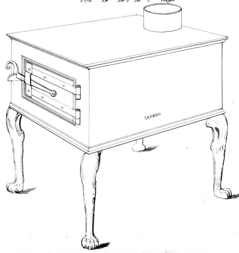
N o 4 with Boiler
