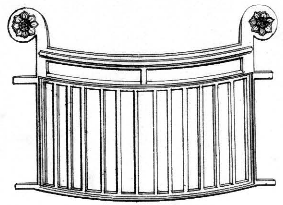
Kilmarnock x Grates. 12, 14, 16, 18, 21, 24 inches wide.
