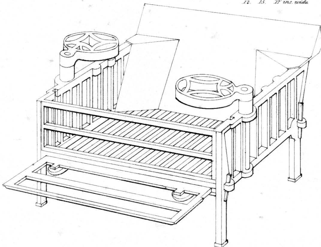
Kentish Cottage Grate N o 1. 2. 3. 12. 15. 17 ins. wide.
