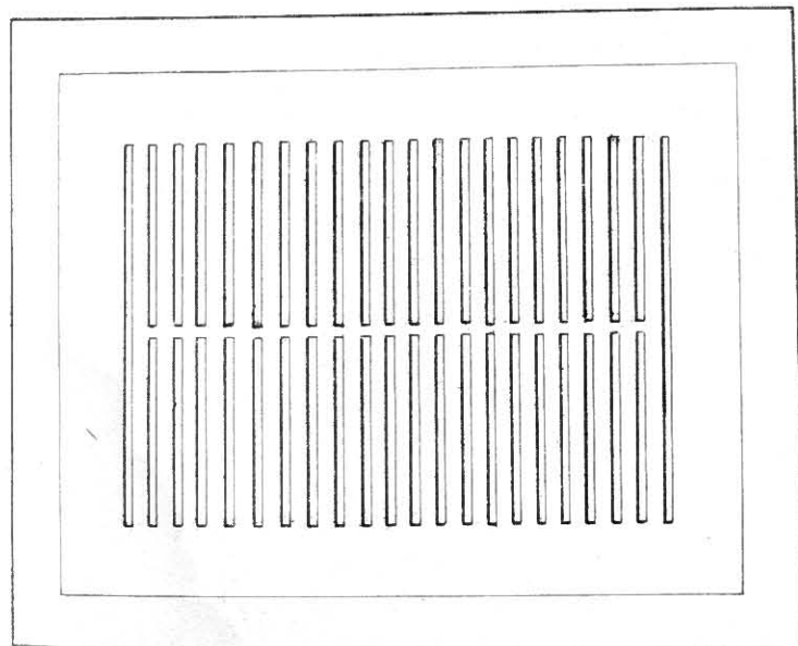
Black or Bright Ash Grate & frame. Sizes outside 14x12 to 24x18 In. Ash Grates only 12 to 28 In. long.
