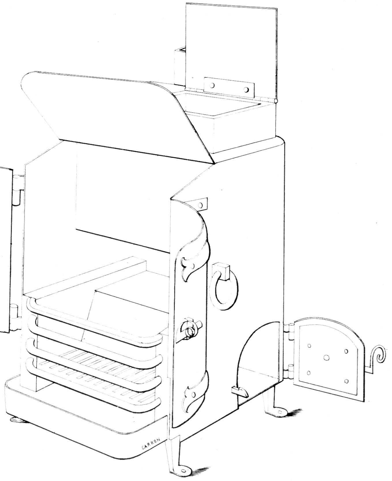
Liverpool Ship Hearths
