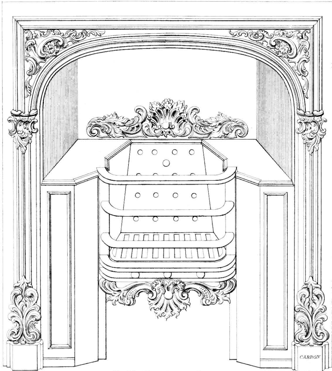
R. E. Register Stove, With N o 15+ Front, N o 10 top Back & N o 20 Fret. Sizes 24, 28, 30, 32 x 30 ins. high.
