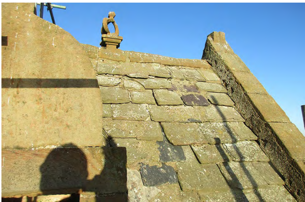
Figure 208: Detail of roof, Tolbooth, Pittenweem, Fife. © Arc Architects.
