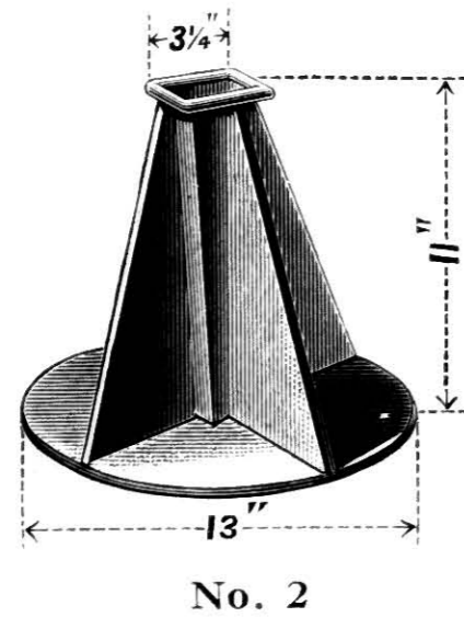
Clothes Post Sockets.
