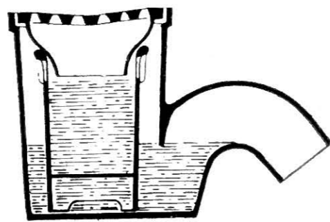
Clark's Patent Trap—Section.
