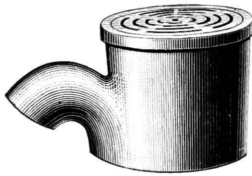
Clark's Patent Trap—Round.
