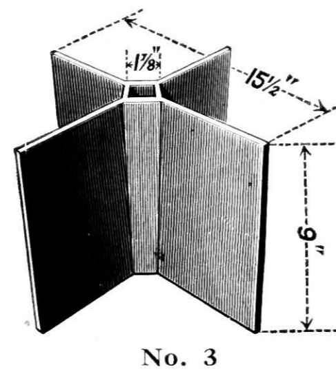
Clothes Post Sockets.
